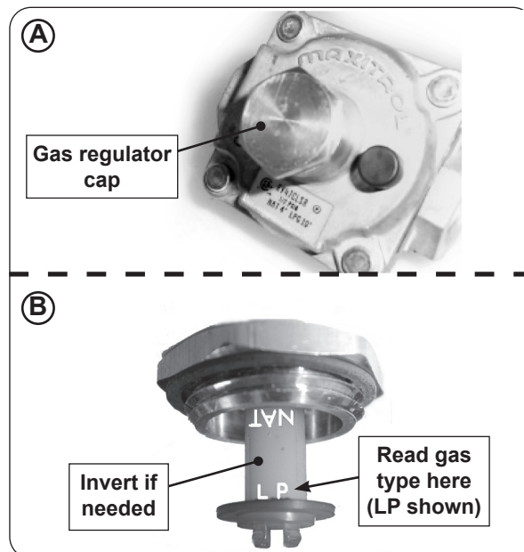
Fig. 44-1 Regulator conversion
