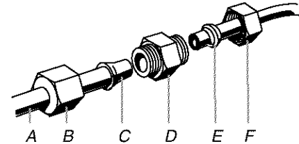
A. Refrigerator water tubing B. Nut (provided) C. Bulb D. Coupling (provided) E. Ferrule (purchased) F. Nut (purchased)
