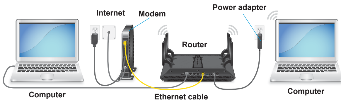
Figure 4. Router cabling
