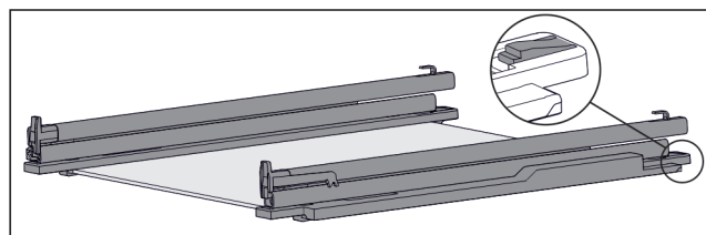
Fig. 128 Glass shelf with rails and retaining parts
