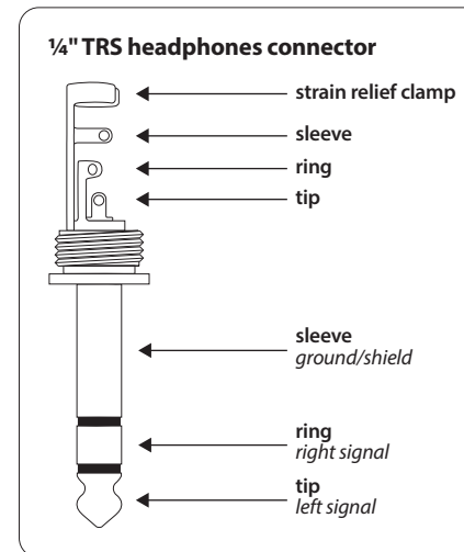
STEREO PLUG FOR HEADPHONES CONNECTION
