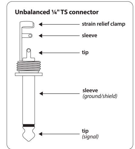
1/4" MONO PLUG
