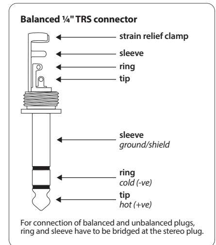
1/4" STEREO PLUG
