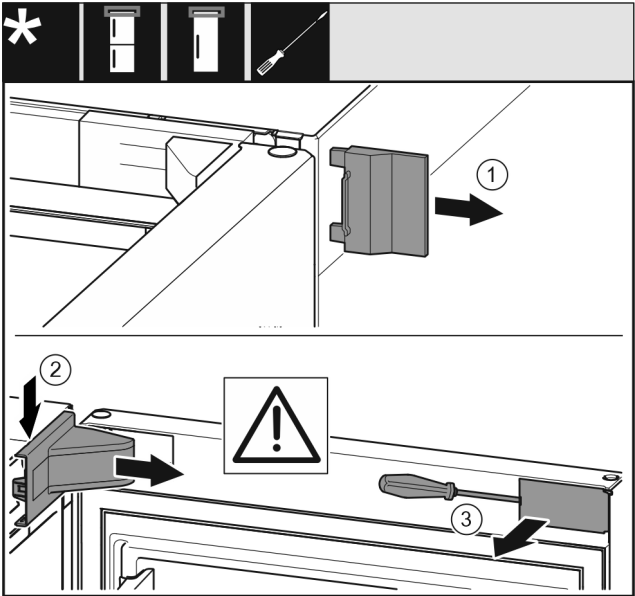
Fig. 8 ► Open the door. ► Remove the outer cover (1). ► Disengage and remove the swap bearing block cover (2).
