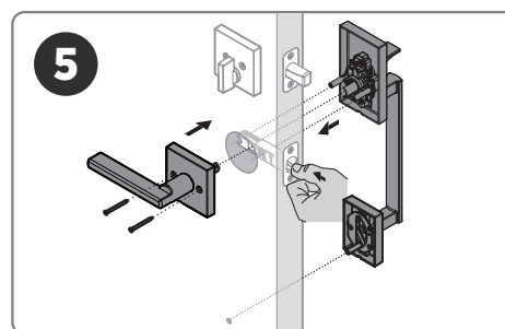
Secure exterior grip and interior lever together with mounting screws
