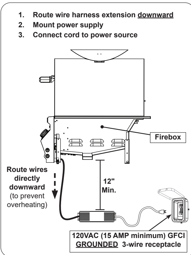
Fig. 28-2 Mount power supply
