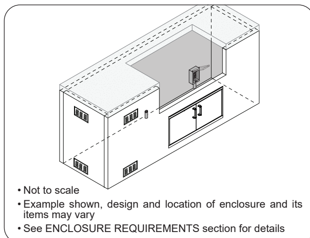
Fig. 27-1 Enclosure construction overview (if applicable)
