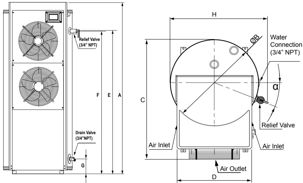
Figure 5. Rough-In Dimensions
