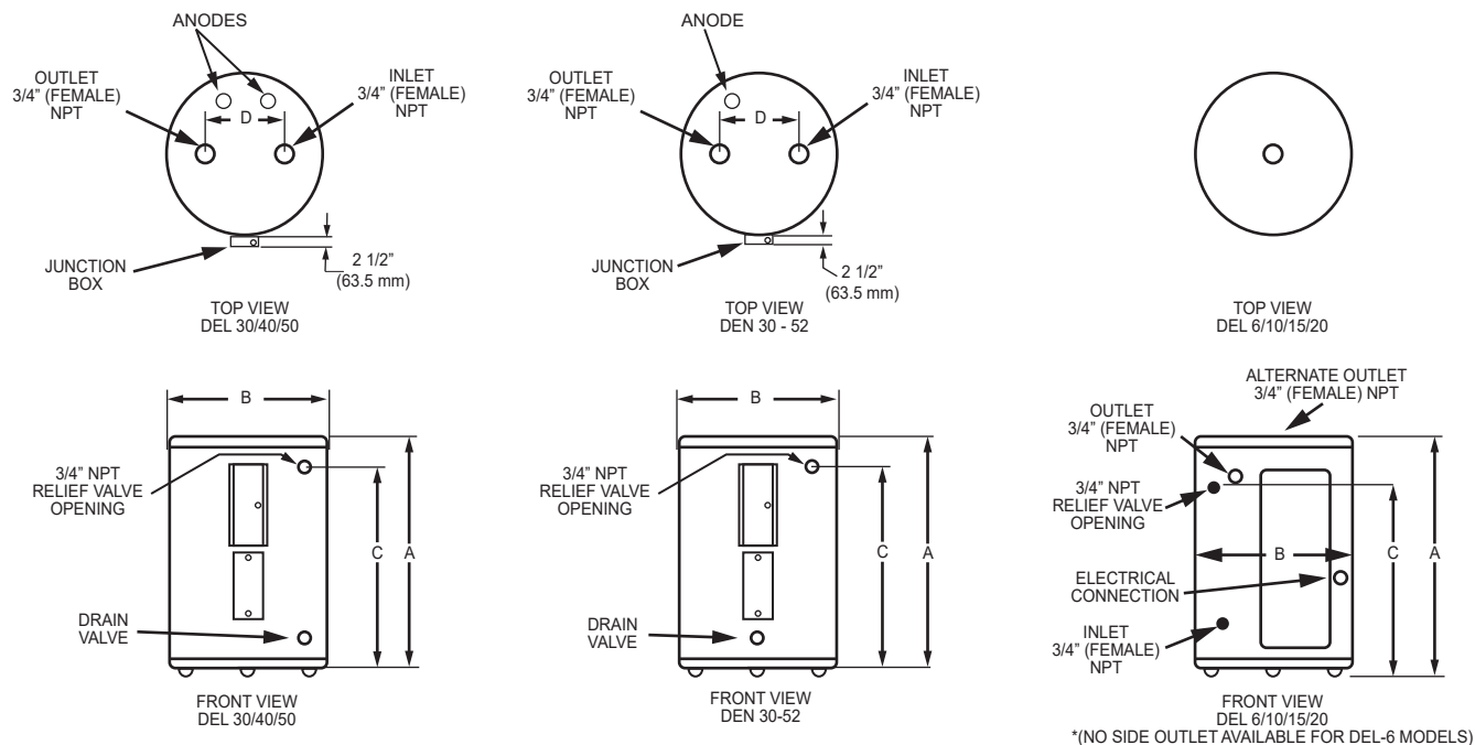
Figure 2. Rough-In Dimensions
