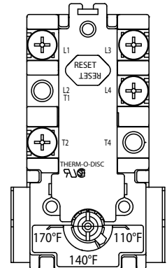
Figure 4. C-2 Thermostat
