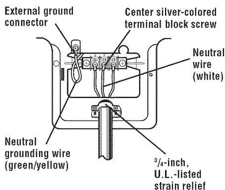
3-Wire Connection with Frame-Grounding Conductor
