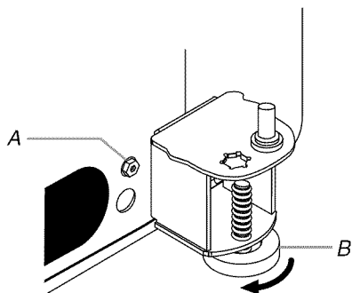
A. Roller adjustment screw B. Brake foot
