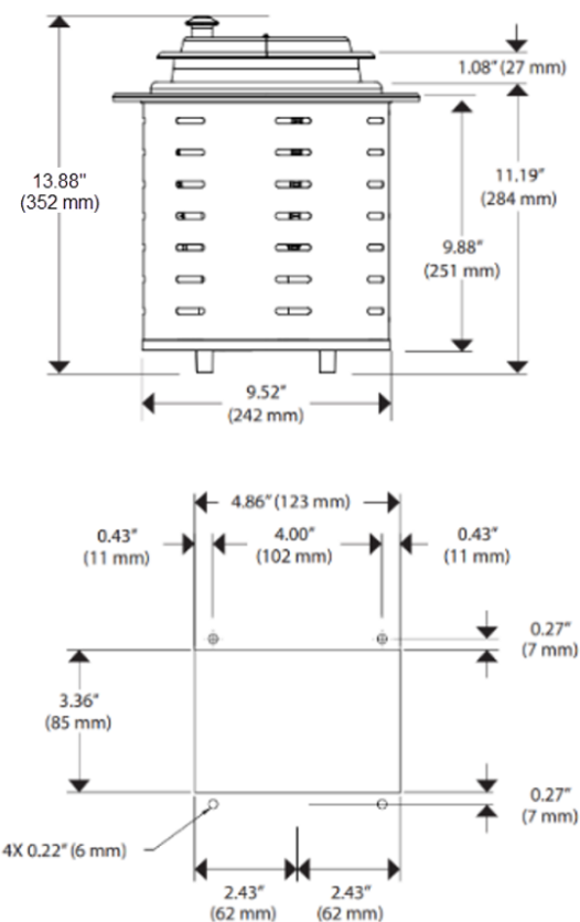
Figure 3-4: 4 Qt Drop-In SinAqua Souper
