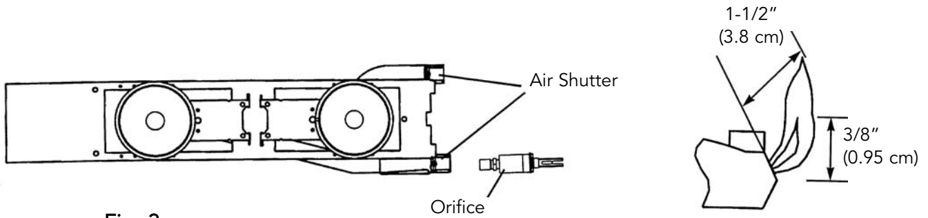
Fig. 3 SIDE BURNER (If applicable)
