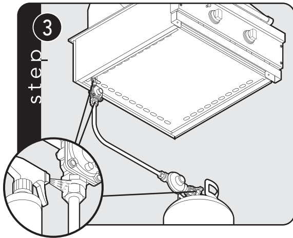
Apply the soap solution to fittings.
