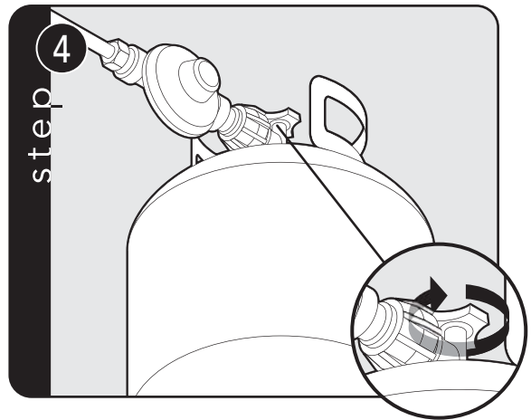
Turn cylinder valve knob counter clockwise one turn to open.
