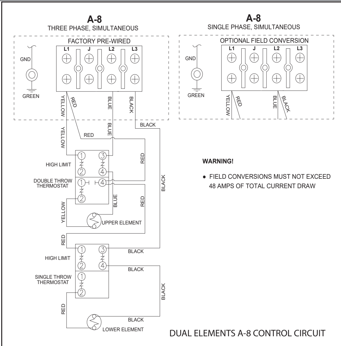
Figure 8. Wiring Diagram
