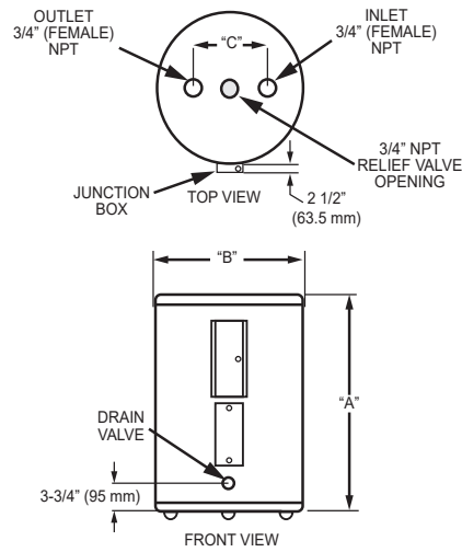
Figure 2. Dimensions and Capacities
