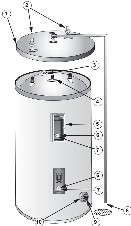
Figure 7. Leakage Checkpoints
