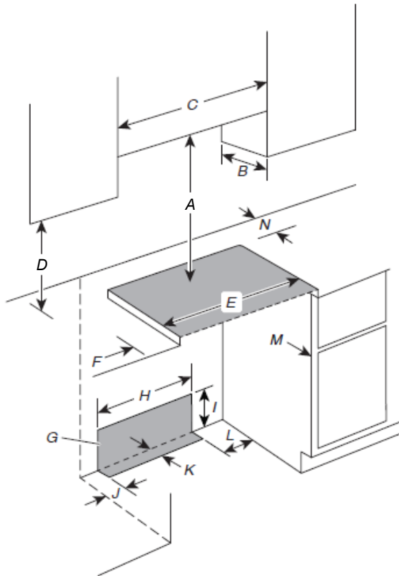
Slide-In Cutout
