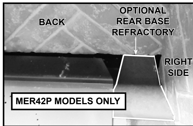
Figure 11.7 MER42P Models Only: Optional Rear Base Refractory Piece Installed (Right Side Shown)
