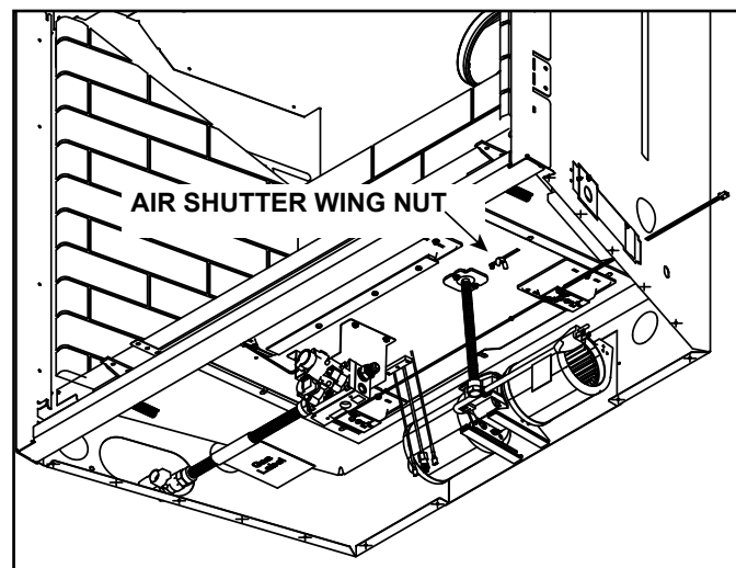
Figure 9.2 Air Shutter
