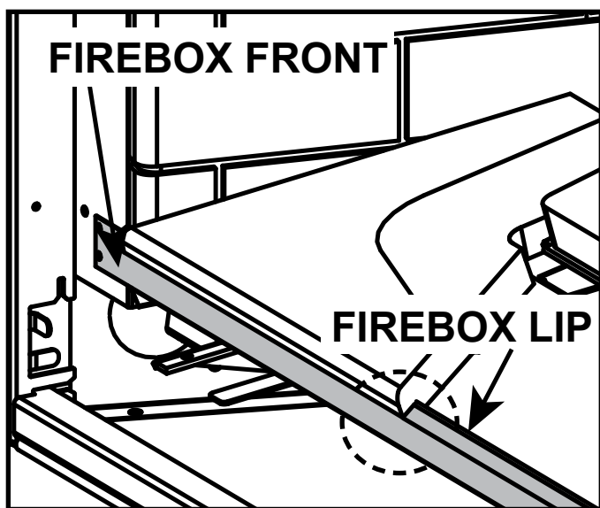
Figure 11.9 Front Base Refractory Installed
