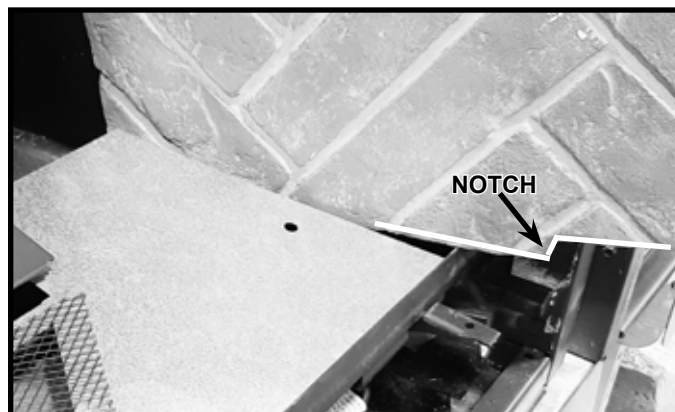
Figure 11.2 Side Refractory Panel Notch
