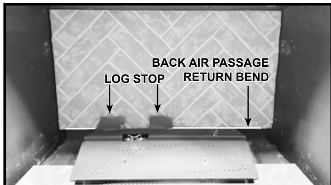
Figure 11.1 Install Back Refractory Panel
