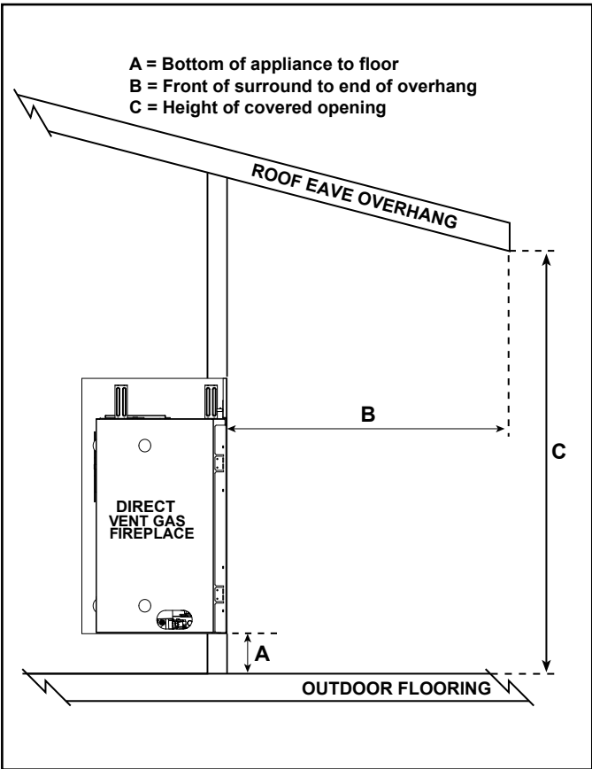
Figure 3.7 Protected Outdoor Applications - Dimensions
