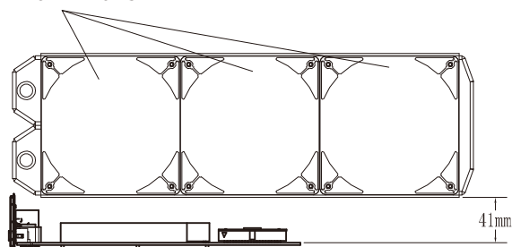
120mm fans
