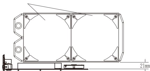
140mm fans
