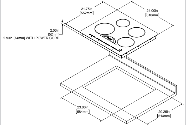
B80405 & B82405
