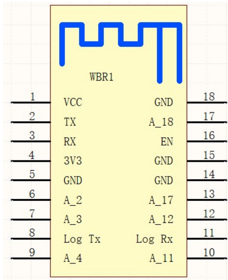
Figure 6-3 WBR1-IPEX pins
