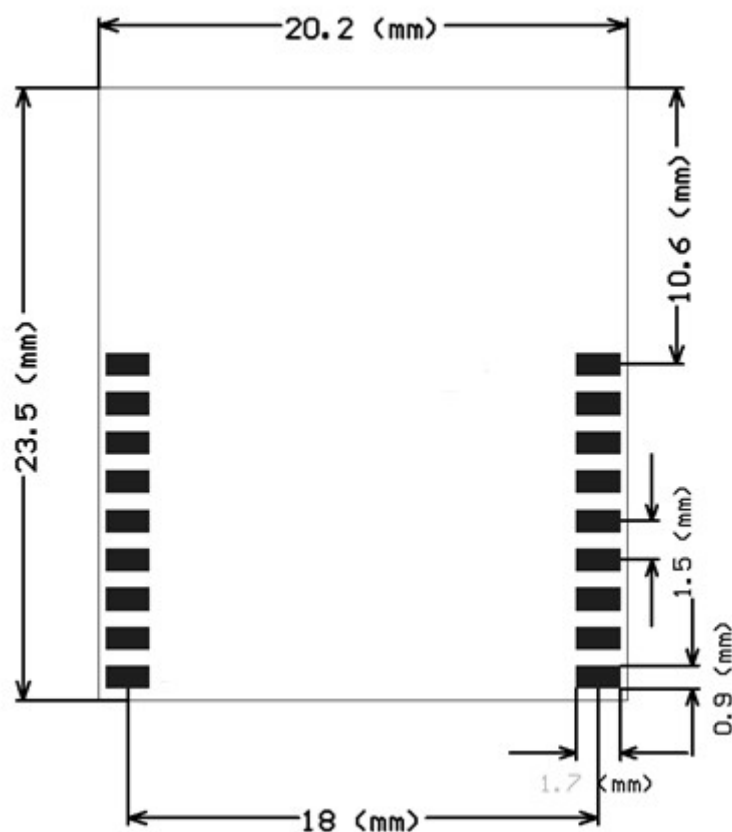
Figure 6-4 Layout of the PCB to which WBR1-IPEX applies
