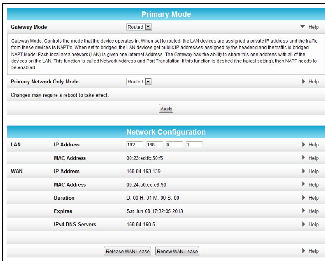
Figure 23 – Basic Setup Screen
