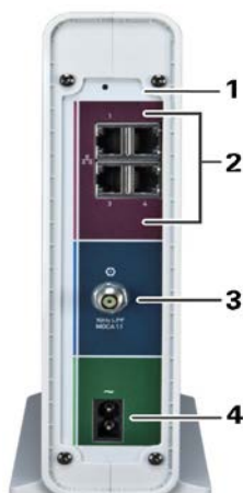
Figure 2 – SBG6782-AC Rear View
