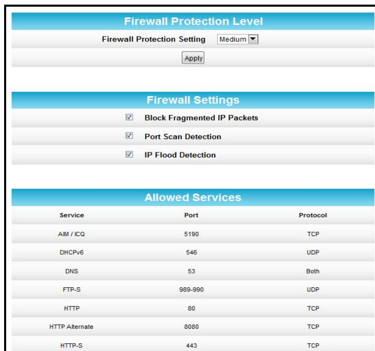
Figure 28 – Firewall Protection Level Screen
