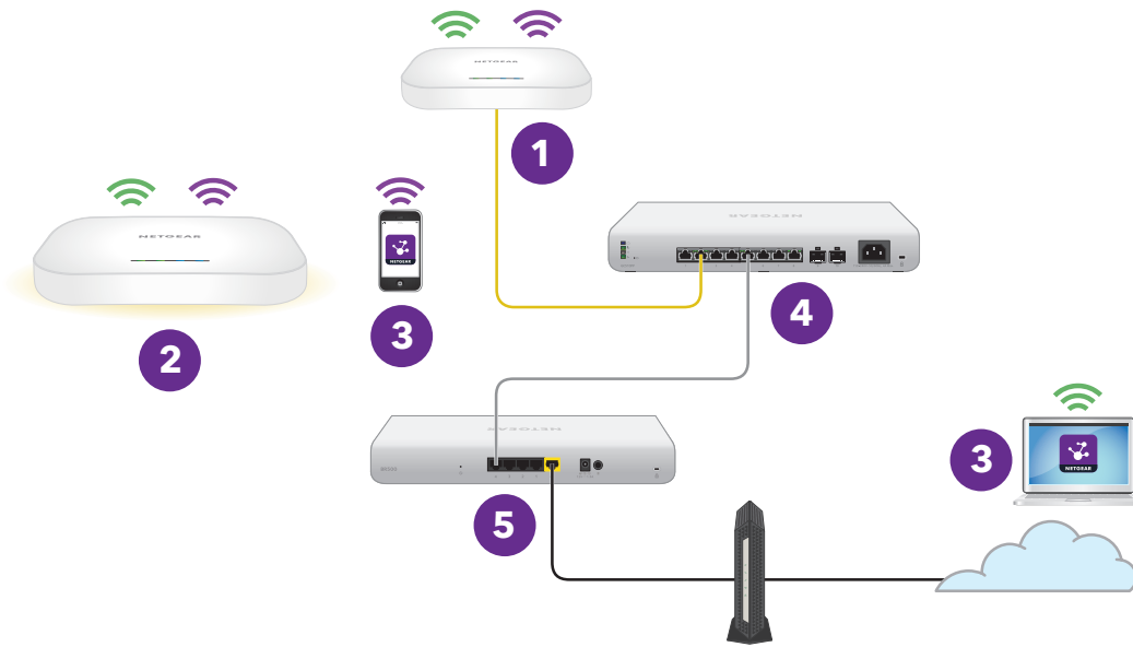
Figure 10. Connect the extender access point to a wired root access point
