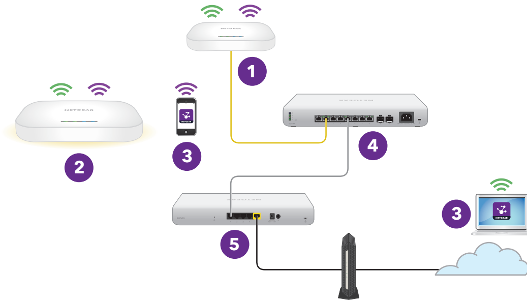
Figure 9. Mesh network with an extender access point and a wired root access point
