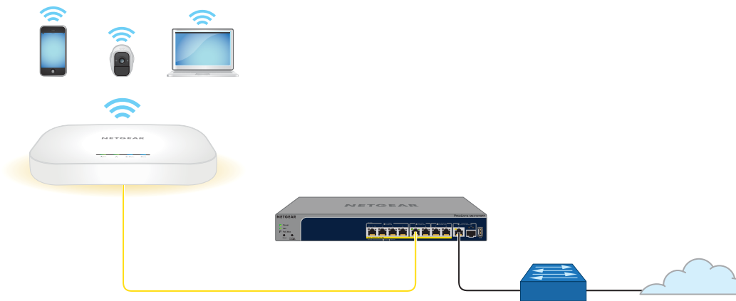
Figure 7. Set up model WAX610 with a PoE+ connection to your network
