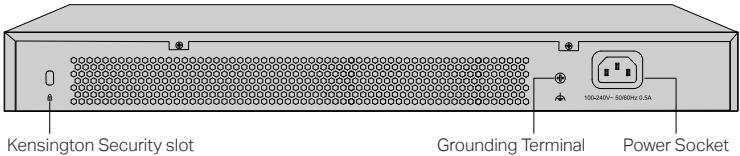
Figure 1-7 Rear Panel
