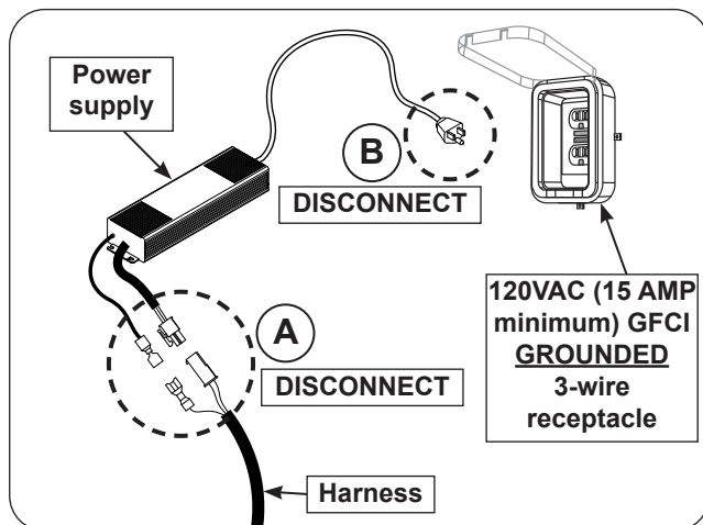
Fig. 45-1 Perform system reset
