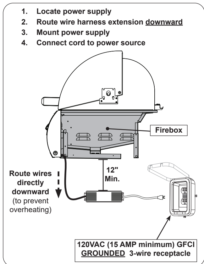
Fig. 30-3 Electrical installation
