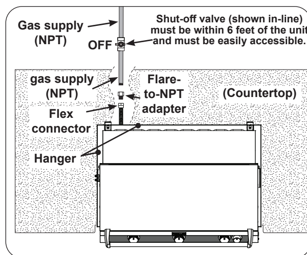
Fig. 31-2 Household LP & Nat. gas diagram
