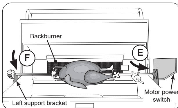
Fig. 39-4 Attach Rotisserie rod to motor
