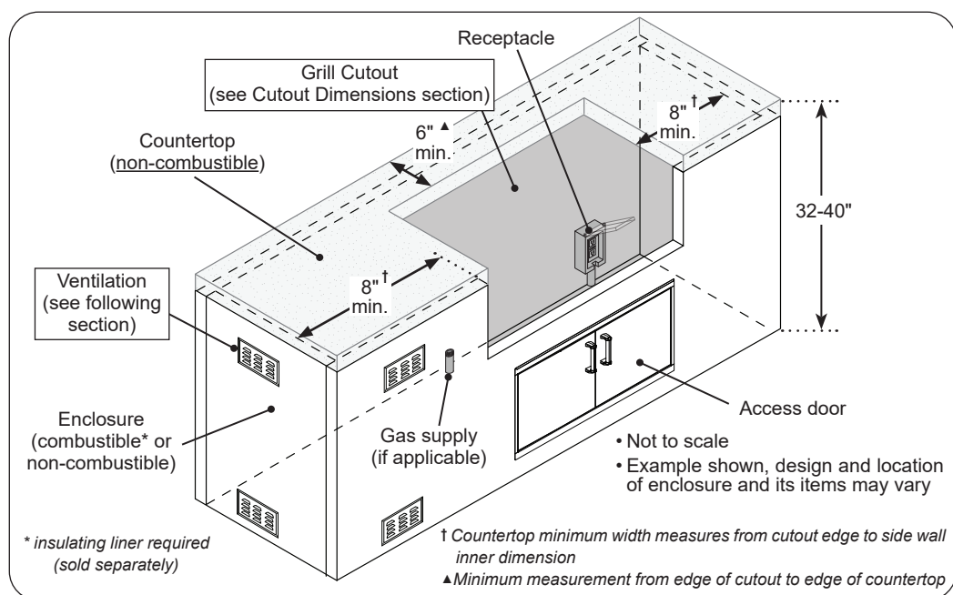
Fig. 11-1 Enclosure specifications
