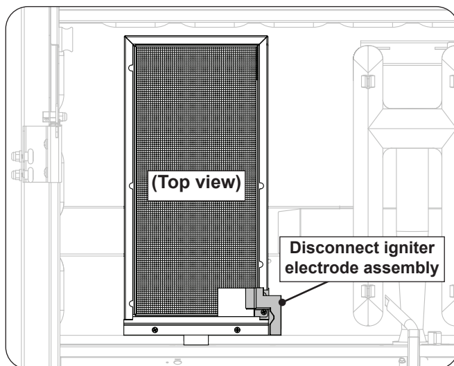
Fig. 45-4 Infrared burner removal
