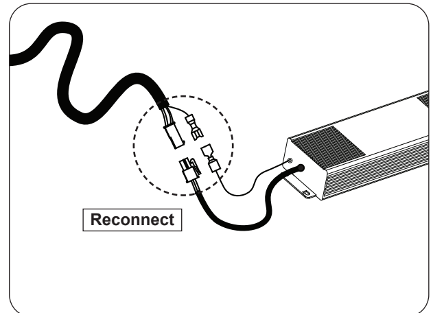
Fig. 30-2 Reconnect harness
