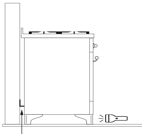
Anti-tip bracket
