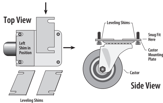
Fig. 6. Install castor shims in pairs.
