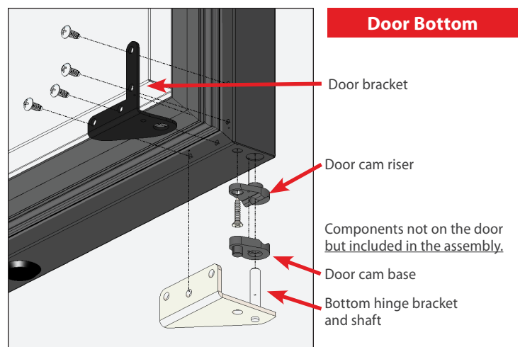
Fig. 4b. Bottom hinge components.
