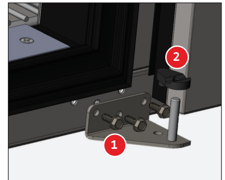
Fig. 9. Install the bottom hinge pin in its new location.
