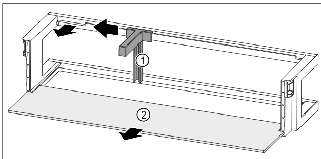
Fig. 133 Door rack with bottle holder and shelf
