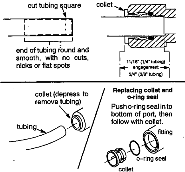
FIG. 11 Tubing correctly cut and connected
