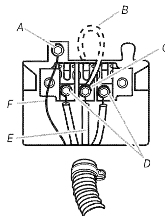
A. External ground conductor screw B. Appliance neutral ground wire C. Center terminal block screw D. Outer terminal block screws E. Neutral (center wire) F. Green or bare ground wire
