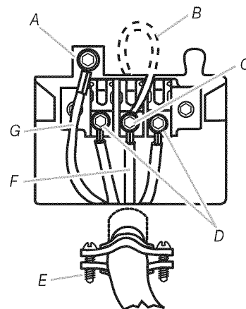
A. External ground conductor screw B. Appliance neutral ground wire C. Center terminal block screw D. Outer terminal block screws E. Strain relief screw F. Neutral (center wire) G. Ground wire
