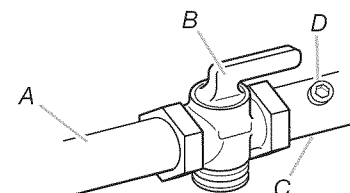
A. Gas supply line B. Shutoff valve in "open" position C. To dryer D. NPT 1/8" min. plugged tapping
