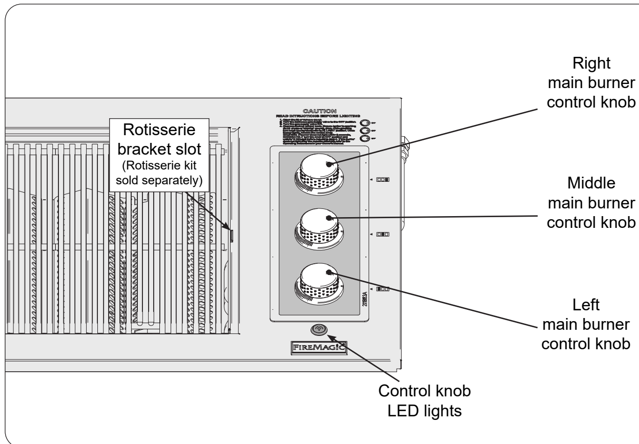
Fig. 34-2 Echelon Diamond countertop grill controls (Open top models)
