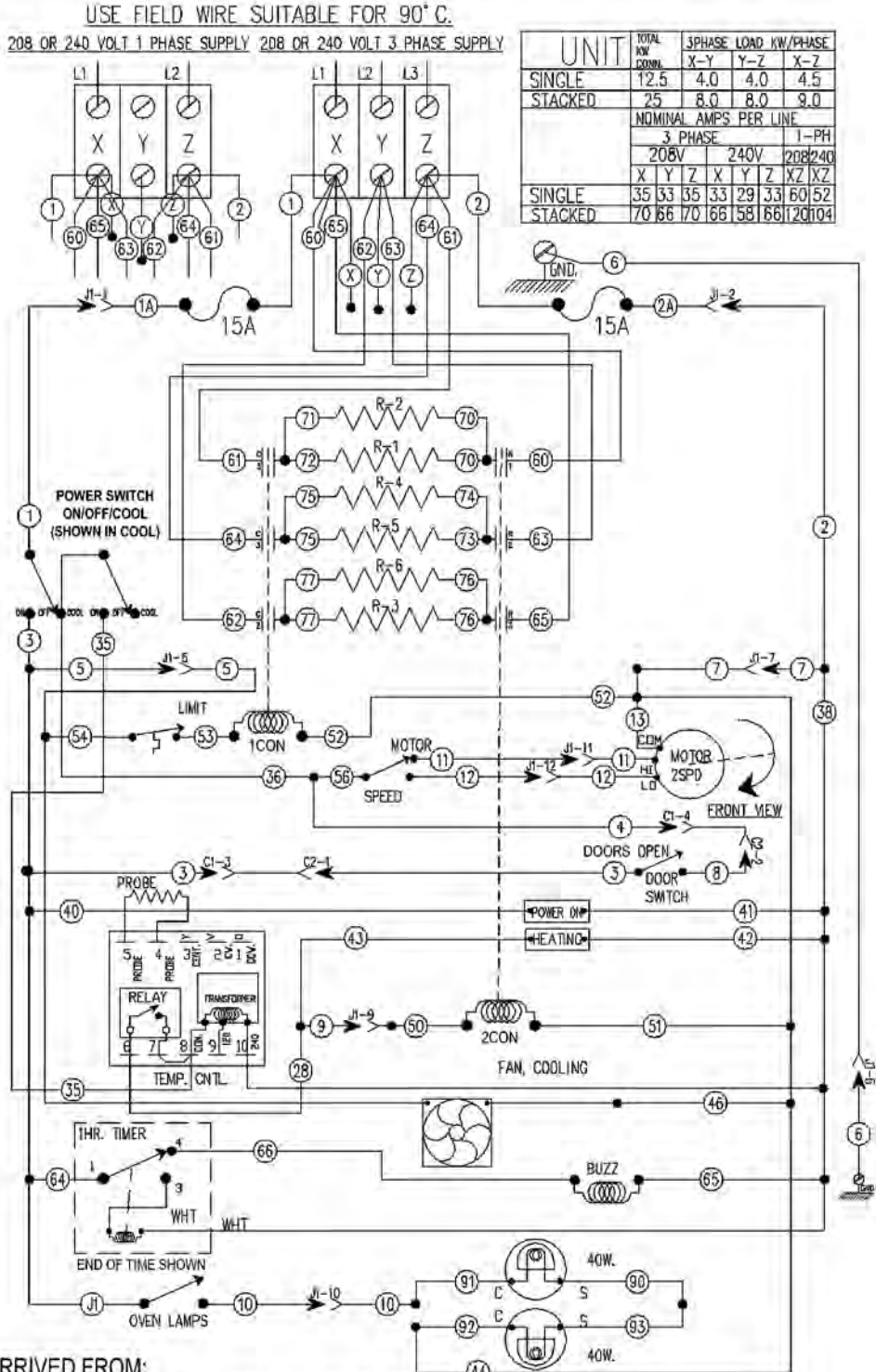
VC4ED, VC6ED with Solid State Temperature Control, 208-240V Schematic
