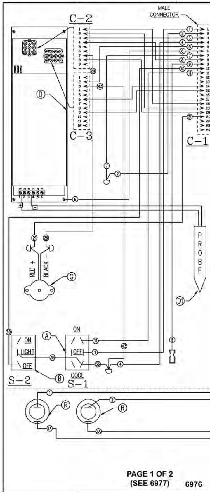
VC4EC, VC6EC Computer Control, 208-240V (Roast & Hold Standard)
