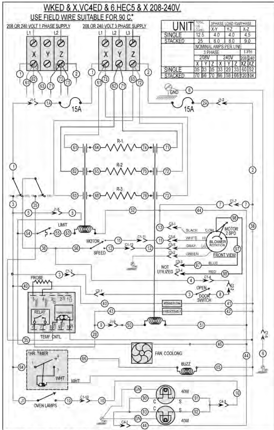
WKED & X, VC4ED & 6, HEC5 & X 208-240V.
