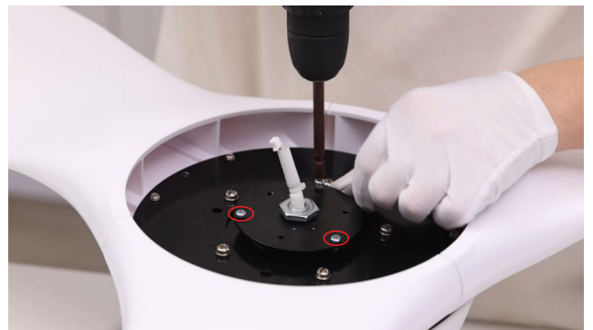
12.Loosen and remove the 3 silver screws pre-locked on the motor (They will be needed later)
