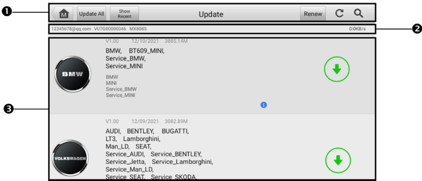
Figure 9-1 Update Screen
