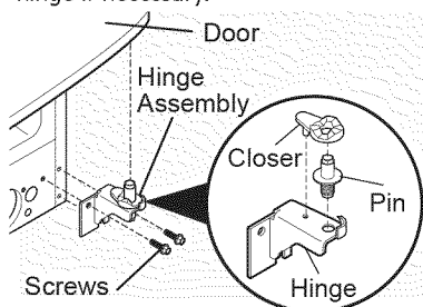
Adjustable Hinge
