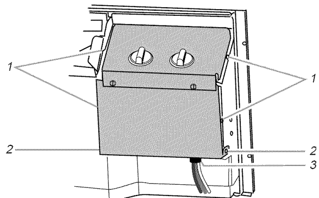
1. Remove these screws. 2. Do not remove these screws. 3. Bushing
