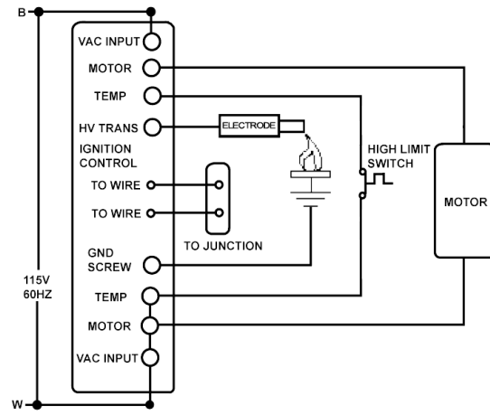
SCHEMATIC DIAGRAM
