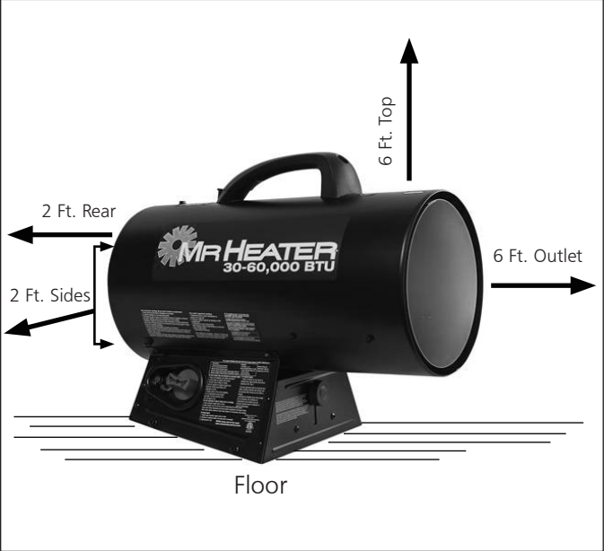
Figure 2 Clearance Diagram
