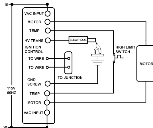
SCHEMATIC DIAGRAM
