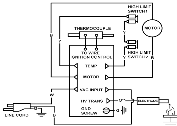
CONNECTION DIAGRAM
