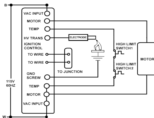
SCHEMATIC DIAGRAM
