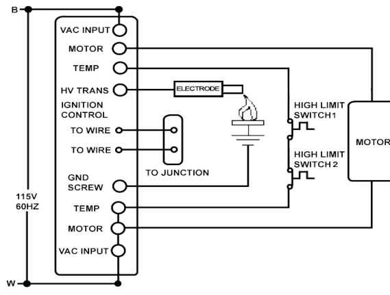
SCHEMATIC DIAGRAM
