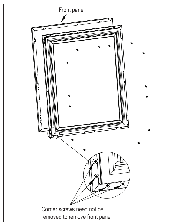
Figure 7: Removing Front Panel
