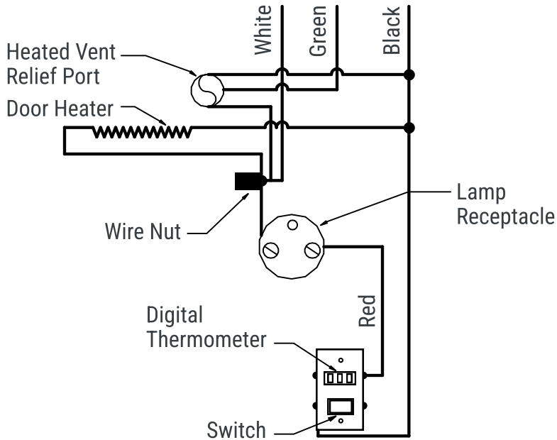
WIRING DIAGRAM
