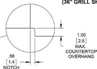
TYPICAL ISLAND INSTALLATION (36" GRILL SHOWN)
