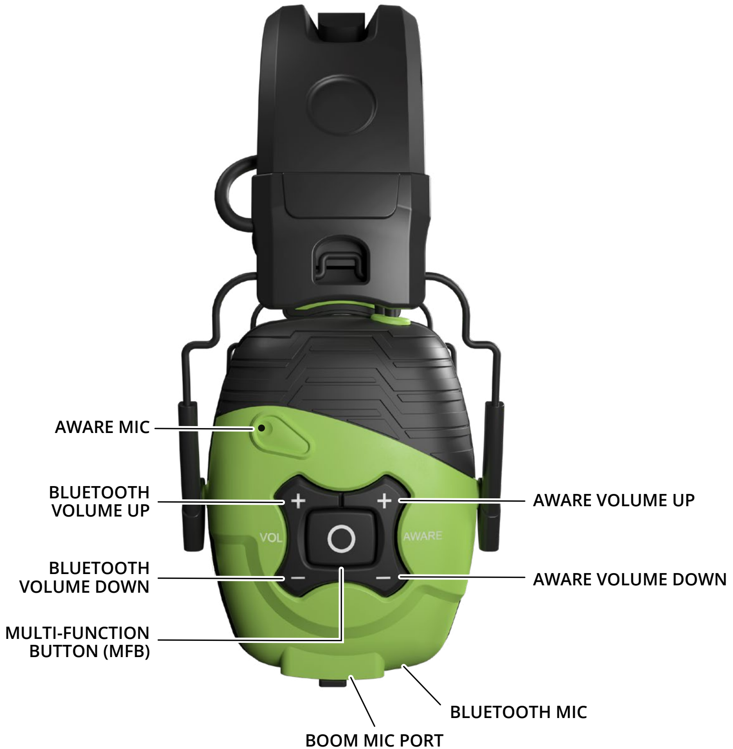
RIGHT EARCUP
