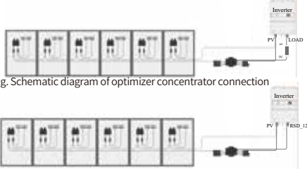
h. Use the RSD port of inverter to supply the concentrator
