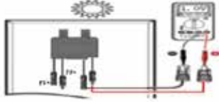
d. Optimizer output detection
