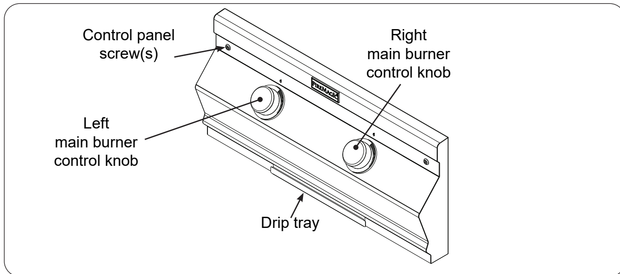
Fig. 30-1 CM430i controls
