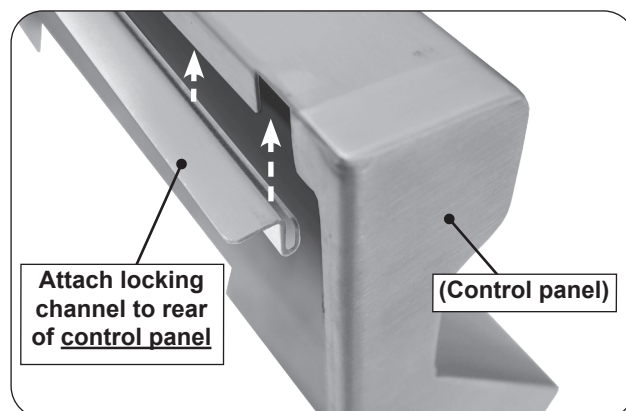
Fig. 28-3 Attach cooking grid locking channel
