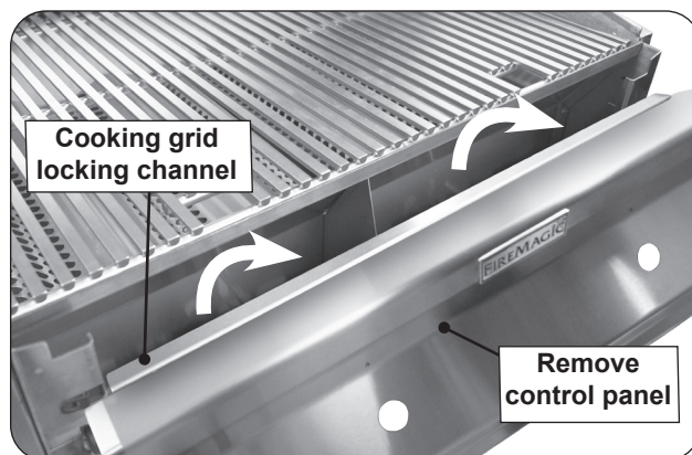
Fig. 37-1 Control panel / grid locking channel removal
