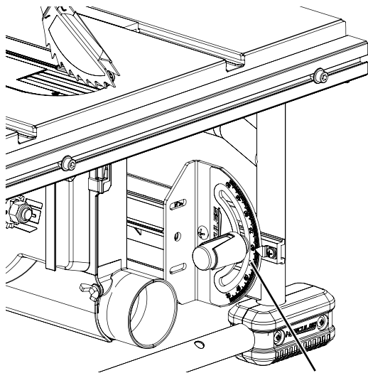
Miter Gauge
