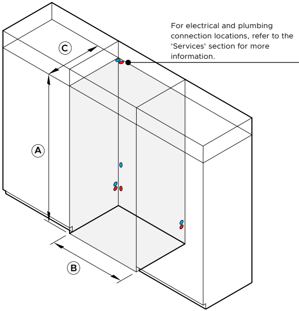
ISOMETRIC VIEW
