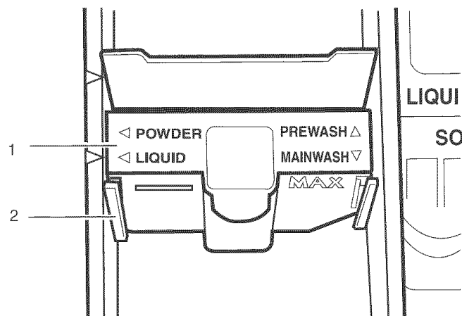
Separator in front position, between guides
