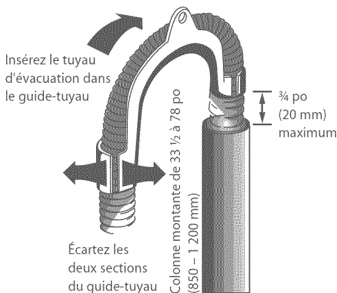
Fig.2 Installation du guide-tuyau
