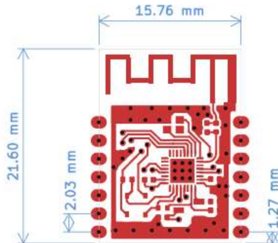
Module Dimension Diagram
