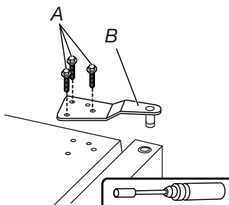
A. Hex Head Screws B. Hinge Pin
