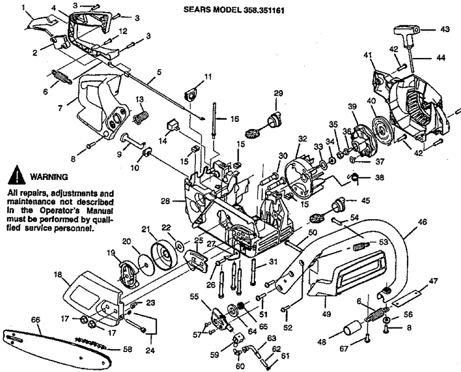
SEARS MODEL 358.351161
